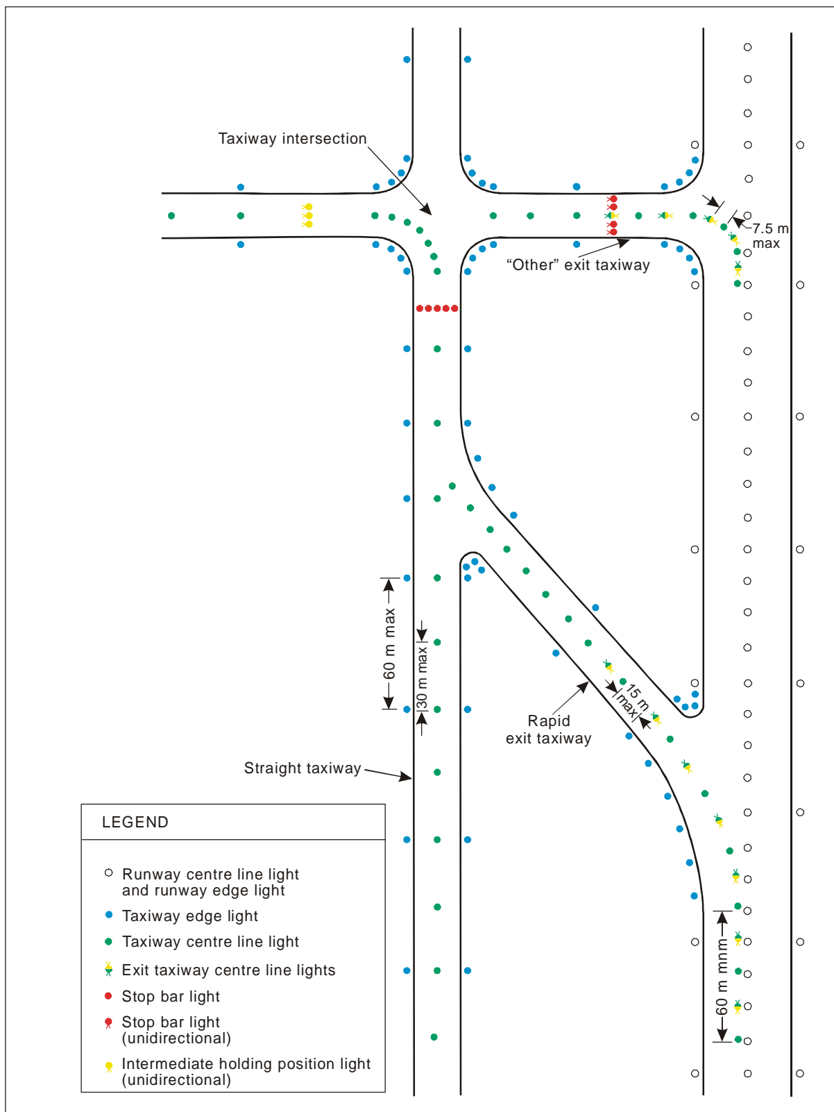
Figure 5-26. Taxiway lighting
