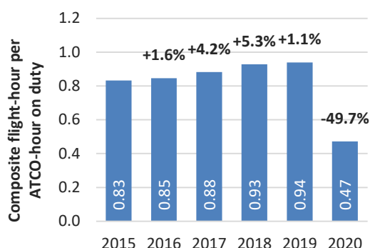
Figure 3.11: ATCO-hour productivity (2015-2020)
